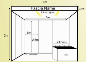
Shell Scheme Perspective View
